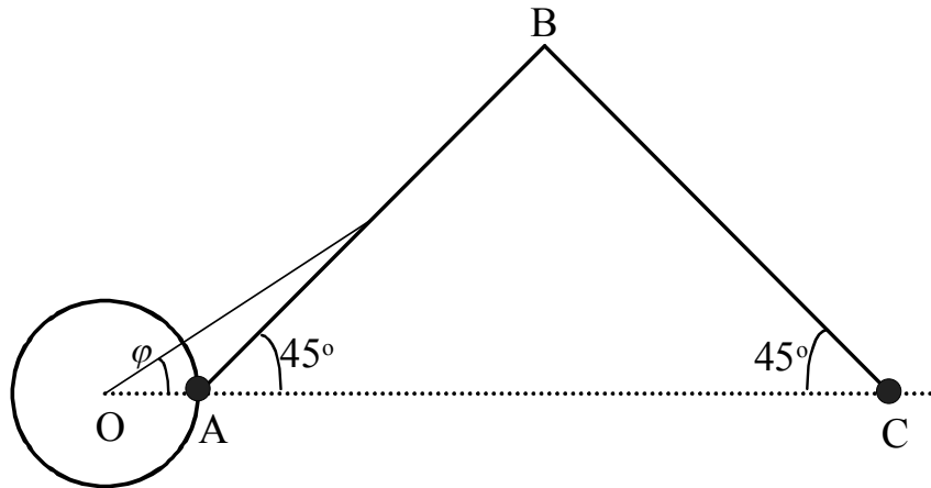
Fig. 6. Scheme of space flight O – centre of Earth A – start of flight C – Moon (finish) AC – projection of gravitational flat
