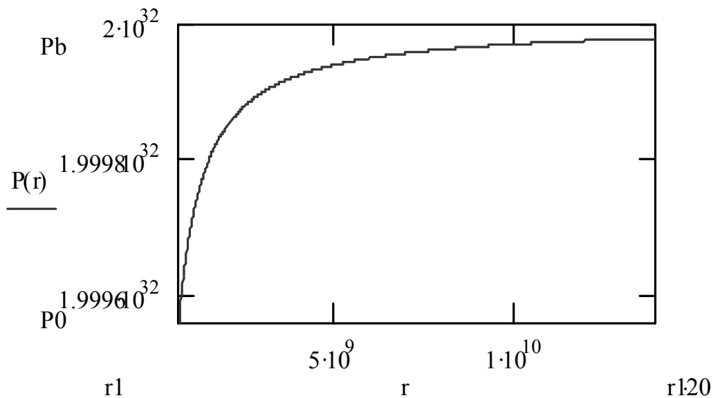
Fig.2. Radial distribution of the ether pressure for the Sun (f.15).
