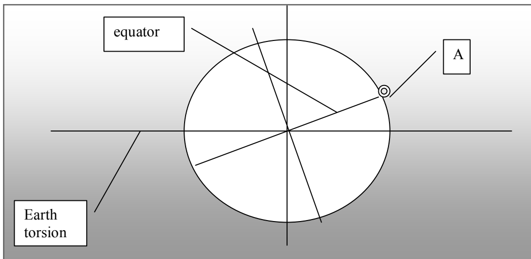
Fig.7 : Inclination of the Earth equator
