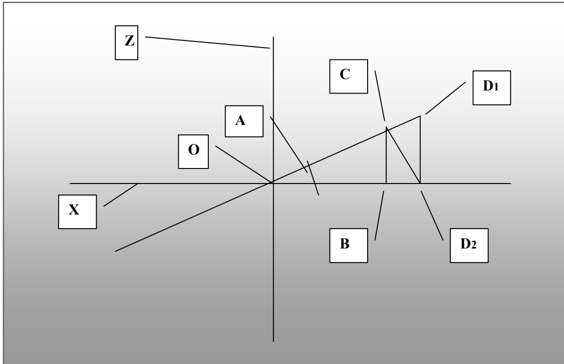
Fig.5. Plane projections of minor and major orbital semi-axes.
