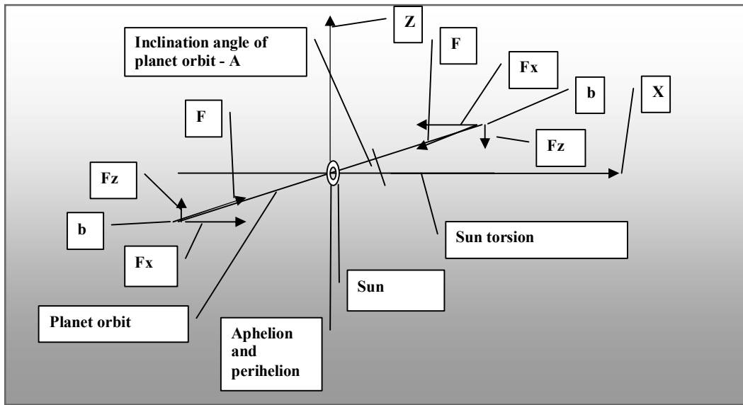
Fig. 3 Kinematical scheme of orbital motion
