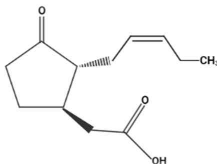
Figure 1 Structure of jasmonic acid
