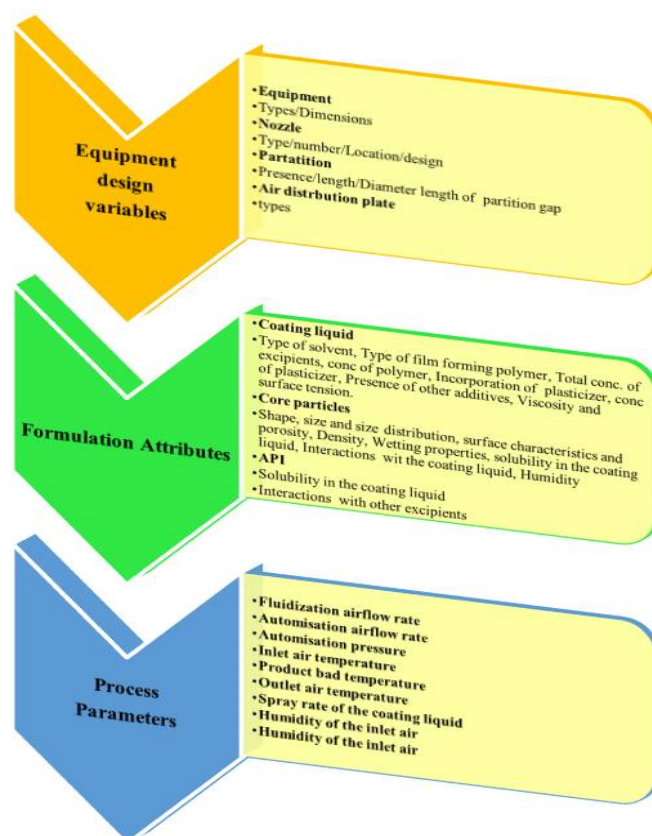
Figure 10: Parameters of the coating process
